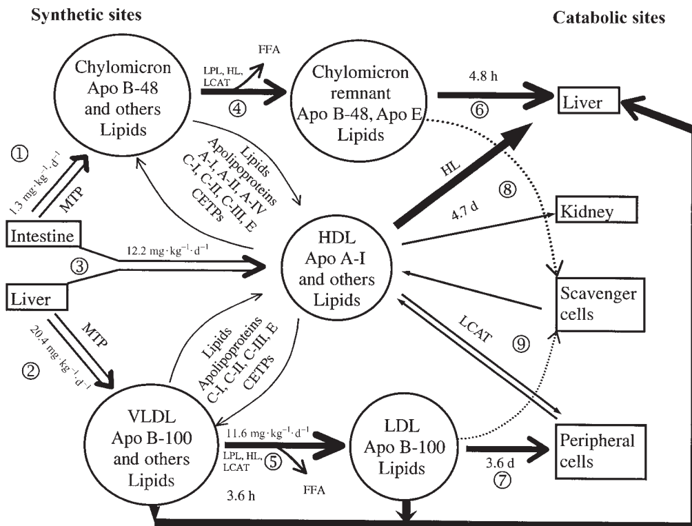
FIGURE 2. An overview of human apolipoprotein (apo) metabolism as assessed by endogenous labeling with a primed constant infusion of deuterated leucine in the fed state. CETP, cholesterol ester transfer protein (transfers cholesterol ester from LDL and HDL to remnants of triacylglycerol-rich lipoproteins); FFA, free fatty acid; HL, hepatic lipase (cleaves fatty acids from both phospholipid and triacylglycerol); LCAT, lecithin cholesterol acyltransferase (phosphatidylcholine-sterol O -acyltransferase; transfers fatty acid from phosphatidyl choline or lecithin to cholesterol to form cholesterol ester); LPL, lipoprotein lipase (cleaves fatty acids from glycerol backbone on triacylglycerol); MTP, microsomal transfer protein (joins lipid with apo B). Open arrows indicate secretion pathways (with secretion rates). Closed arrows indicate catabolic pathways (with mean residence times for apo B-48, apo A-I, and apo B-100, respectively). See references 31 and 32.
